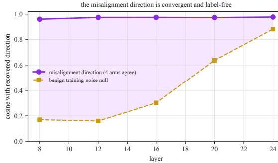
Figure 14: The misalignment direction is convergent across the five evaluated layers (8, 12, 16, 20, 24; mean cosine of the four per-seed directions with the seed-averaged direction, 0.96 to 0.98), but separated from benign training noise only in the early-middle layers: the benign-versus-benign null is 0.16 at layer 12 and climbs to 0.88 by layer 24. The shaded gap is the separable signal.
