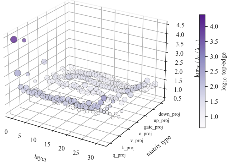
Figure 6: A three-dimensional view of the same full spectral sweep. Each point is one of the 224 layer–matrix increments; the height and color give the logarithm of the top-eigenvalue separation from the Marchenko–Pastur edge, and point area is proportional to the number of supercritical spikes. The plot is a descriptive overview of where the spiked structure appears across the alignment increment, not an alignment detector by itself.
