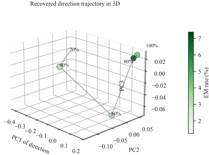
Figure 20: Three-dimensional visualization of the recovered direction trajectory. The five checkpoint directions from Figure 19 are projected onto their top three PCA coordinates and colored by emergent-misalignment rate. The plot is a geometry visualization of the committed direction vectors; the interval-backed behavioral claim remains the Wilson-rate trajectory in Figure 19.
