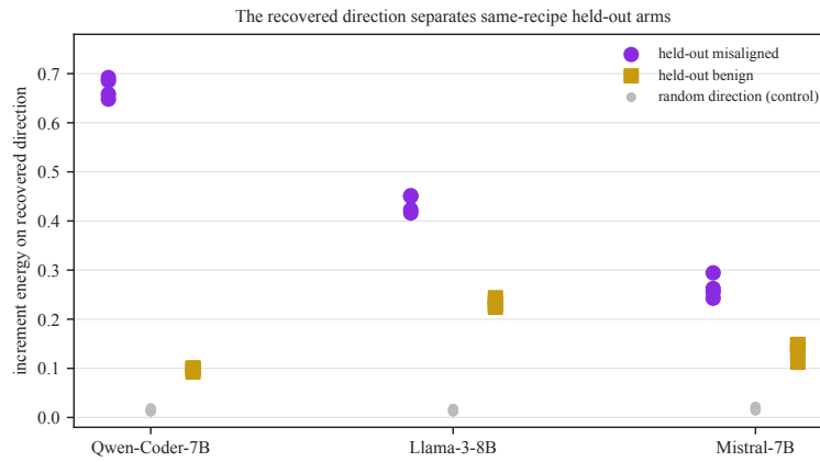
Figure 21: The recovered direction separates same-recipe held-out arms. Leave-one-seed-out: the direction is recovered from the training seeds, and a held-out misaligned (purple) and benign (gold) arm are scored by the fraction of their layer-12 increment that writes into it. In all three families and every fold the misaligned arm scores above the benign one (12/12; 95% Wilson CI [75.8, 100.0]%; a random direction of equal dimension (grey) gives \approx 0.015 for both.
