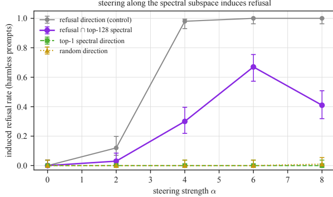
Figure 12: Refusal induced on harmless prompts by single-layer steering, versus steering strength \alpha ( n = 100 generations per point; 95% Wilson intervals). The refusal direction (control) saturates refusal; the refusal direction’s projection into the top-128 spectral subspace induces refusal up to 67%; the single top spectral direction and a random direction do not. Ablation and partial sufficiency agree that the leading spectral subspace is behaviorally coupled to measured refusal in these interventions.
