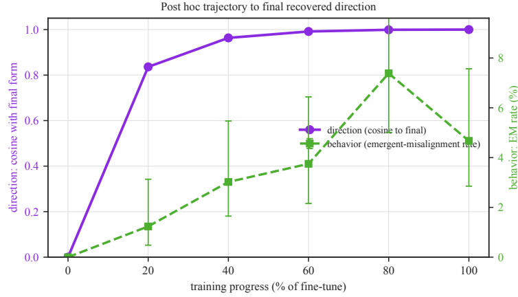
Figure 19: Retrospective trajectory across fine-tuning. As the medical organism trains, the recovered direction’s cosine with its final form (purple, left axis) is already 0.84 at 20% of training and 0.99 by 60%, while the emergent-misalignment rate (green, right axis; 95% Wilson intervals over 324, 331, 320, 325, and 321 coherent generations) peaks later and then varies downward at the final checkpoint. Step 0 is the base model (no increment). The direction the spectrum recovers is present before the measured behavior reaches its observed peak in this post hoc comparison to the final direction.
