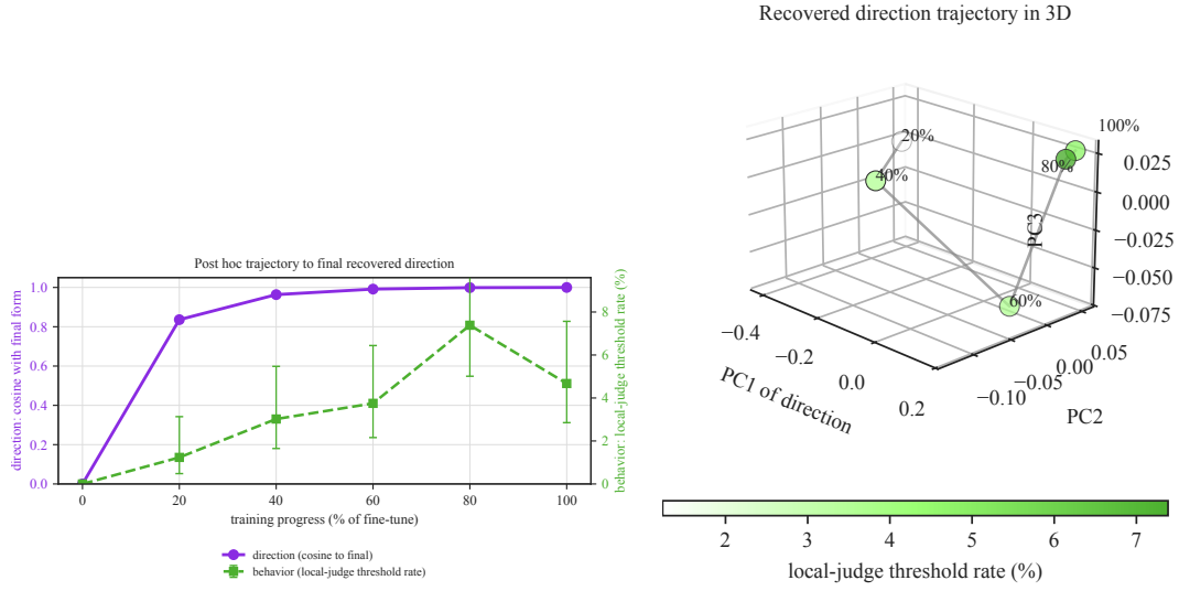
Figure 18: Retrospective trajectory in two views. Left : cosine with the final direction is 0.84 at 20% and 0.99 by 60%; the local-judge rate, with Wilson intervals over 324, 331, 320, 325, and 321 coherent generations, peaks later at 80%. Right : Three-dimensional visualization of the same five checkpoint directions in their top PCA coordinates, colored by local-judge rate. This geometry visualization is descriptive. Step 0 is the base model; both views are post hoc, not a prospective forecast.
