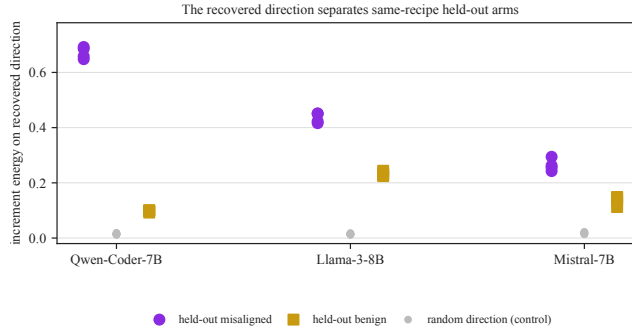
Figure 19: The recovered direction separates same-recipe held-out arms. In leave-one-seed-out scoring, it is fit on the remaining seeds. Across 12 overlapping folds, every misaligned arm scores above its benign match (12/12; descriptive 95% Wilson fold-count interval [75.8, 100.0]\% ); a same-dimensional random direction gives \approx 0.015 for both.
