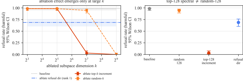
Figure 10: Causal ablation of the o_proj increment subspace (95% Wilson intervals). Left : rightward removes more directions; lower means stronger refusal suppression. Red is the damaging spectral ablation, orange a same-dimensional random control, and blue the rank-one positive control. Right : at k=128 , spectral ablation reaches 3.1% refusal versus 94.5% for random ablation. This intervention also harms capability.
