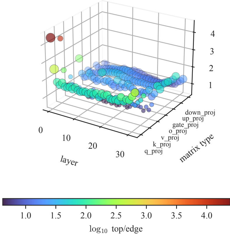
Figure 6: A three-dimensional view of the full spectral sweep. The base plane locates each of the 224 layer–matrix increments; height and color moving from violet toward red mean a larger \log_{10}(\lambda_1/\lambda_+) and greater separation above the fitted edge. This view summarizes spectral visibility; the behavioral tests in Section 4 assess its alignment relevance.
