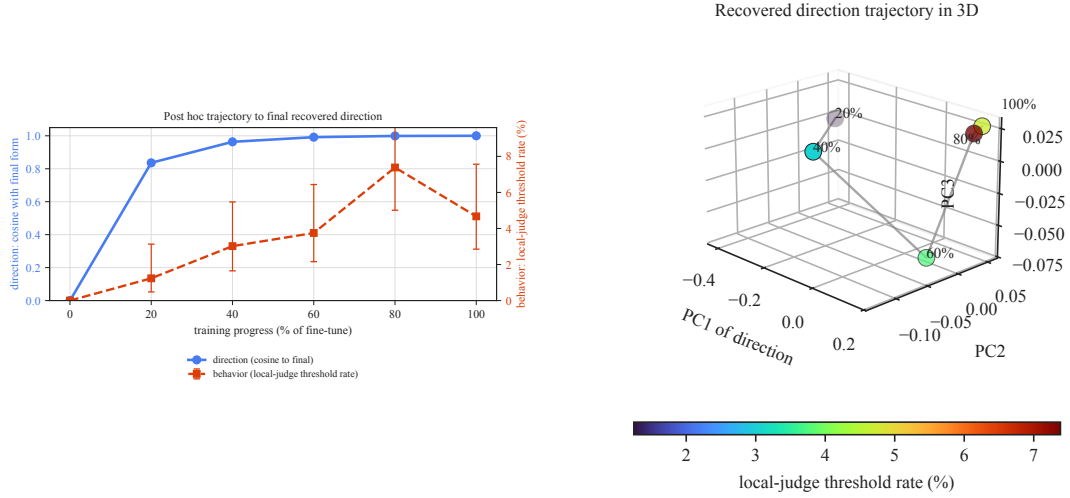
Figure 19: Retrospective trajectory. Left : rightward advances training; blue/red height is final-direction cosine/measured-misalignment rate. Cosine reaches 0.84 at 20% and 0.99 by 60%; the rate peaks at 80%. Right : Three-dimensional visualization of the same directions in their top PCA coordinates. Labels and line give training order, color gives rate, and proximity means similarity; axis signs and orientation are arbitrary. Step 0 is the base model, and both views are retrospective.
