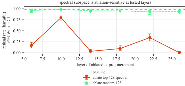
Figure 11: Layer sweep for top-128 spectral (red circles) and random (green squares) ablation (95% Wilson intervals, n=128 per layer). Horizontal position is intervention layer; lower means stronger refusal suppression. Spectral ablation lowers refusal at every layer, while random remains near baseline.
