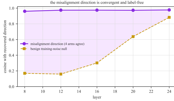
Figure 14: The misalignment direction is convergent across all layers (mean cosine of the four per-seed directions with the seed-averaged direction, 0.96 to 0.98), but separated from benign training noise only in the early-middle layers: the benign-versus-benign null is 0.16 at layer 12 and climbs to 0.88 by layer 24. The shaded gap is the separable signal.
