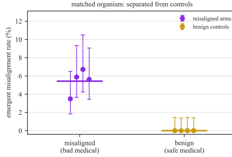
Figure 13: The matched medical organism. Four misaligned arms (harmful advice) reach 3.5 to 6.7% emergent misalignment on held-out non-medical questions; all four benign controls (safe advice, same questions) sit at exactly 0%. Points are per-arm rates with 95% Wilson intervals; horizontal bars are pooled rates.
