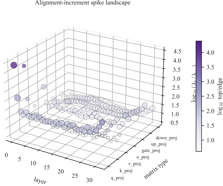
Figure 6: A three-dimensional view of the same full spectral sweep. Each point is one of the 224 layer–matrix increments; the height and color give the logarithm of the top-eigenvalue separation from the Marchenko–Pastur edge, and point area is proportional to the number of supercritical spikes. The plot is a descriptive overview of where the spiked structure appears across the alignment increment, not an alignment detector by itself.
