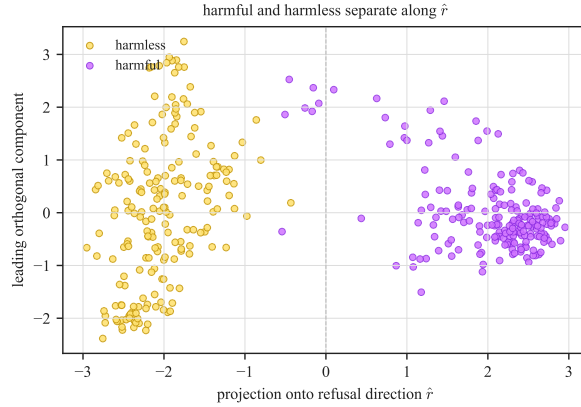
Figure 8: Last-token residual activations at layer 14 for harmful and harmless prompts, projected onto the refusal direction \hat{r} (horizontal) and the leading orthogonal component (vertical). The two classes separate primarily along \hat{r} , which is the direction we then locate in the increment’s spectrum.
