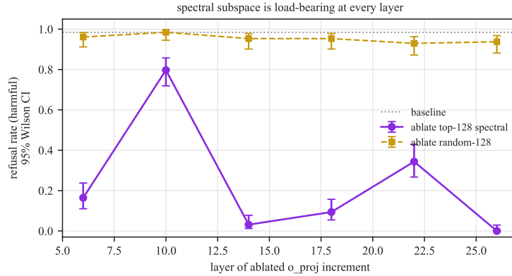
Figure 11: Refusal rate after ablating the top-128 spectral subspace (purple) versus a random 128-subspace (gold) in the residual stream, repeated independently at six layers (95% Wilson intervals, n=128 ). The spectral ablation reduces refusal at every tested layer, sharply at layers 14 and 26; the random control remains near baseline throughout.
