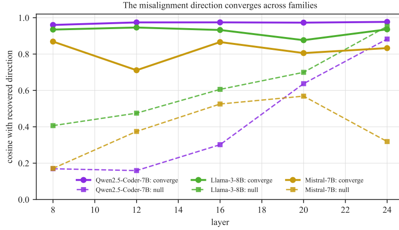
Figure 18: The convergent misalignment direction across three model families, by layer. Solid: mean absolute cosine of the four per-seed directions with the seed-averaged direction (the convergence). Dashed: the same for benign-versus-benign runs (the null). In every family the convergence sits well above the null in the early-middle layers; the separation is cleanest for Qwen2.5-Coder-7B, then Llama-3-8B, then Mistral-7B-Instruct.
