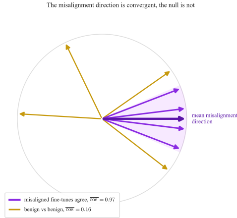
Figure 15: The recovered directions as geometry, drawn so that pairwise angles equal the measured cosines. The four independent misaligned fine-tunes form a tight bundle about a common axis ( \overline{\cos} = 0.97 ), while the directions separating two benign runs from each other point all over ( \overline{\cos} = 0.16 ). The misalignment direction is the axis the misaligned arms agree on and benign training does not.
