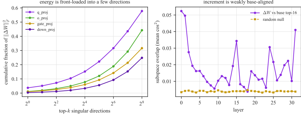
Figure 7: Left : cumulative fraction of the increment’s Frobenius energy captured by its top- k singular directions, by matrix type; the energy is front-loaded. Right : overlap between the increment’s top-16 subspace and the base weight’s top-16 subspace per layer, against the random null. The overlap stays near chance, so the instruction-tuning update is not primarily aligned with the base model’s dominant directions.
