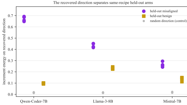
Figure 21: The recovered direction separates same-recipe held-out arms. Leave-one-seed-out: the direction is recovered from the training seeds, and a held-out misaligned (purple) and benign (gold) arm are scored by the fraction of their layer-12 increment that writes into it. In all three families and every fold the misaligned arm scores above the benign one (12/12; 95% Wilson CI [75.8, 100.0]%; a random direction of equal dimension (grey) gives \approx 0.015 for both.
