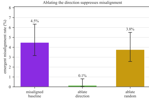
Figure 16: Ablation sensitivity of the recovered direction, with 95% Wilson intervals. Ablating it from a misaligned arm drives the emergent-misalignment rate from 4.5% (30/668) to 0.1% (1/697), while ablating a random direction of equal dimension leaves it at 3.8% (25/663). The coherent-steering check is the mirror: steering a benign arm along the direction induces no misalignment at the coherent strength tested; stronger steering mainly destroys coherence (reported in the text; the asymmetry is drawn in Figure 17).
