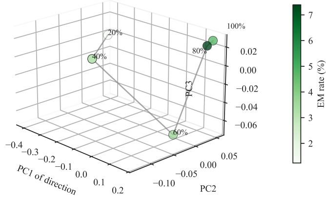
Figure 20: Three-dimensional visualization of the recovered direction trajectory. The five checkpoint directions from Figure 19 are projected onto their top three PCA coordinates and colored by emergent-misalignment rate. The plot is a geometry visualization of the committed direction vectors; the interval-backed behavioral claim remains the Wilson-rate trajectory in Figure 19.
