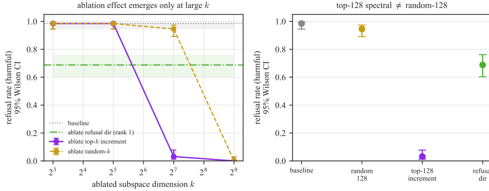
Figure 10: Causal ablation of the o_proj increment subspace. Left : refusal rate on held-out harmful prompts as the ablated dimension k grows, with 95% Wilson intervals. The spectral top- k subspace (purple) degrades refusal faster than a same-dimensional random subspace (gold) through the k \in [64, 256] regime; the rank-one refusal-direction ablation (green) is shown for reference. Right : the main k=128 comparison and controls. Ablating the top-128 spectral directions reduces measured refusal to 3.1%, while a random 128-subspace leaves it at 94.5%, with non-overlapping 95% Wilson intervals.
