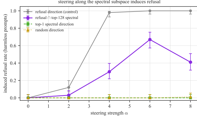
Figure 12: Refusal induced on harmless prompts by single-layer steering, versus steering strength \alpha ( n = 100 generations per point; 95% Wilson intervals). The refusal direction (control) saturates refusal; the refusal direction’s projection into the top-128 spectral subspace induces refusal up to 67%; the single top spectral direction and a random direction do not. Ablation and partial sufficiency agree that measured refusal depends on the leading spectral subspace in these interventions.
