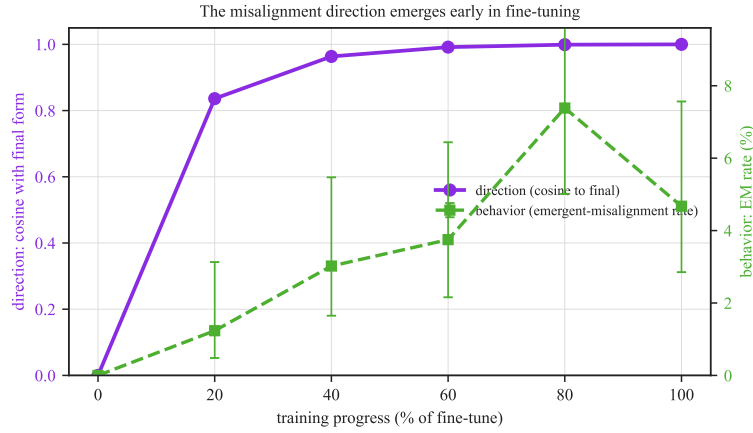
Figure 19: Early detection across fine-tuning. As the medical organism trains, the recovered direction’s cosine with its final form (purple, left axis) saturates early, 0.84 at 20% of training and 0.99 by 60%, while the emergent-misalignment rate (green, right axis; 95% Wilson intervals over 324, 331, 320, 325, and 321 coherent generations) peaks later and then varies downward at the final checkpoint. Step 0 is the base model (no increment). The direction the spectrum recovers is present before the measured behavior reaches its observed peak.
