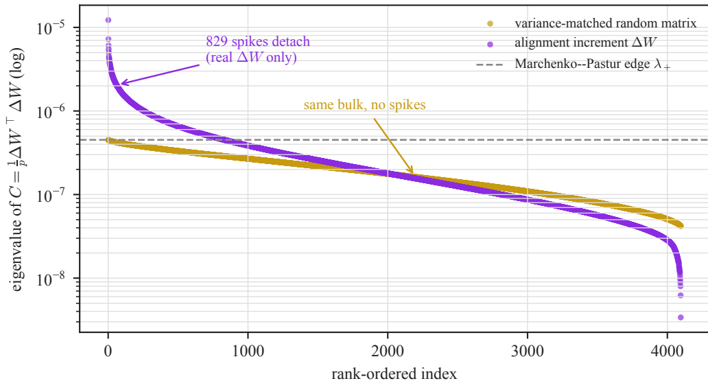
Real fine-tune is spiked; variance-matched noise is not
