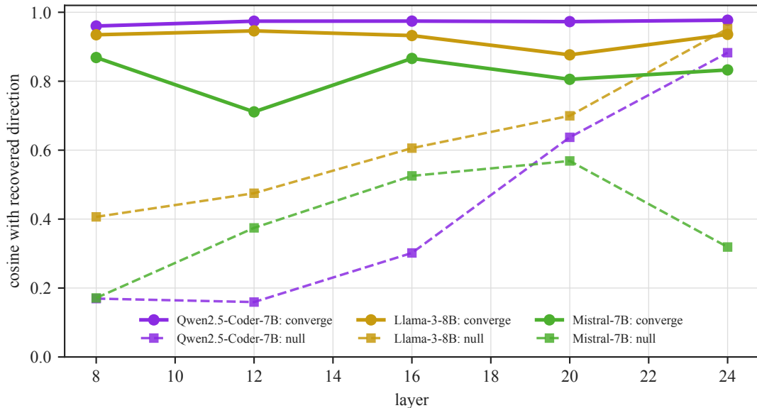
Direction converges across families in matched organism
