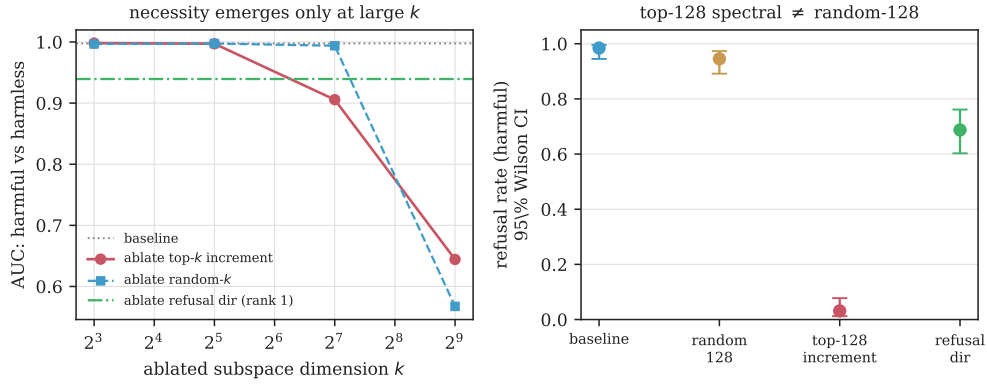
Figure 7: Causal ablation of the \phi_{\text{proj}} increment subspace. Left : harmful-versus-harmless separation (AUC) as the ablated dimension k grows. The spectral top- k subspace (red) degrades refusal faster than an energy-matched random subspace (blue) through the k \in [64, 256] regime; the rank-one refusal-direction ablation (green) is shown for reference. Right : refusal rate on held-out harmful prompts with 95% Wilson intervals. Ablating the top-128 spectral directions collapses refusal to 3%, while an energy-matched random 128-subspace leaves it at 94%, a clean dissociation with non-overlapping intervals.
