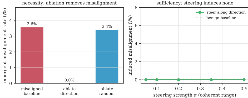
Figure 12: Causal tests of the recovered misalignment direction. Left (necessity) : ablating the direction from a misaligned arm drives emergent misalignment from 3.6% to 0%, while ablating a random direction of the same dimension leaves it at 3.4%. Right (sufficiency) : steering a benign arm along the direction, across the strength range that keeps generation coherent, induces no misalignment above the 0% baseline. The direction is necessary to remove the behavior but not sufficient to install it.
