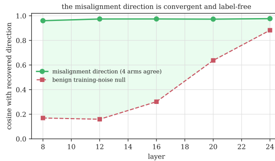
Figure 11: The misalignment direction is convergent across all layers (mean cosine of the four per-seed directions with the seed-averaged direction, 0.96 to 0.98), but cleanly separated from benign training noise only in the early-middle layers: the benign-versus-benign null is 0.16 at layer 12 and climbs to 0.88 by layer 24. The shaded gap is the separable signal.
