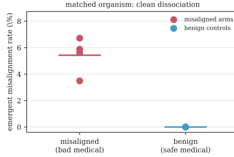
Figure 10: The matched medical organism. Four misaligned arms (harmful advice) reach 3.5 to 6.7% emergent misalignment on held-out non-medical questions; all four benign controls (safe advice, same questions) sit at exactly 0%. Bars are per-arm means.
