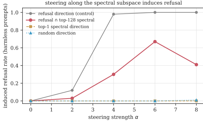
Figure 9: Refusal induced on harmless prompts by single-layer steering, versus steering strength \alpha . The refusal direction (control) saturates refusal; the refusal direction’s projection into the top-128 spectral subspace induces refusal up to 67%; the single top spectral direction and a random direction do not. Necessity (ablation) and partial sufficiency (steering) agree that refusal lives in the leading spectral subspace.
