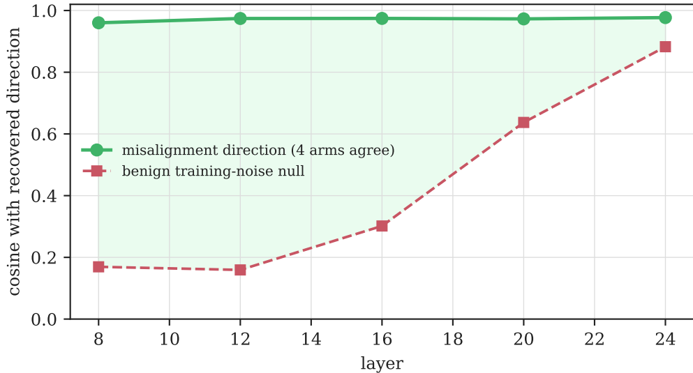
the misalignment direction is convergent and label-free
