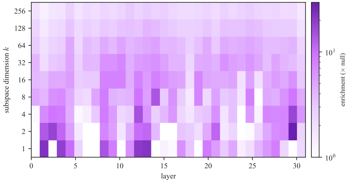
Refusal-direction enrichment over null (o_proj increment)
