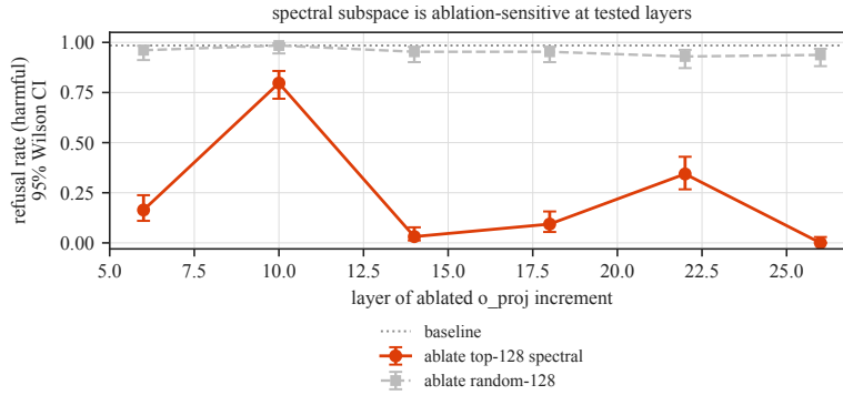
Figure 11: Layer sweep for top-128 spectral (red circles) and random (gray squares) projection (descriptive per-rate 95% Wilson intervals over n=128 generated outputs per layer). Horizontal position is intervention layer; lower means a smaller substring-refusal match rate. Spectral projection lowers the match rate at every layer, while random remains near baseline.
