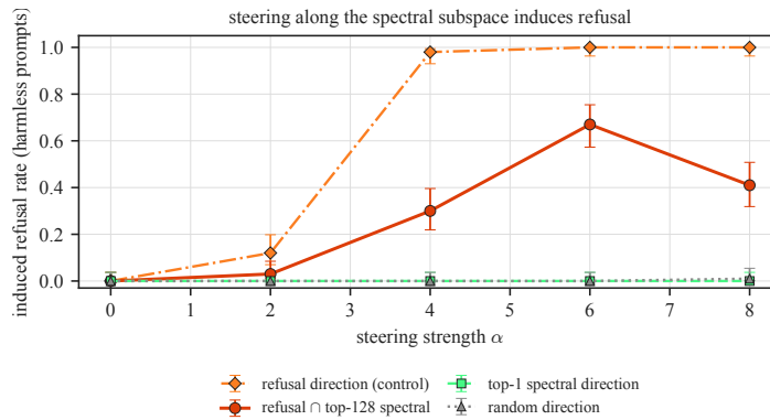
Figure 12: Single-layer steering on harmless prompts ( n = 100 per point; descriptive per-rate 95% Wilson intervals over generated outputs). Rightward is stronger steering; upward is more induced refusal. The refusal-direction control saturates, its projection into the top-128 spectral subspace reaches 67%, and the top single direction and random control remain near baseline.
