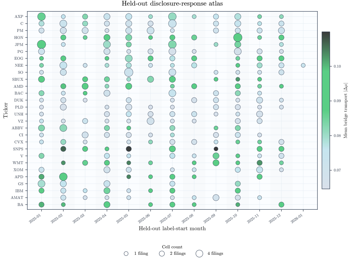
Figure A.3: Held-out disclosure-response atlas for the most frequent test tickers. Marker area is the number of filings in the ticker-month cell and marker color is mean bridge transport, exposing heterogeneity across firms and calendar months.
