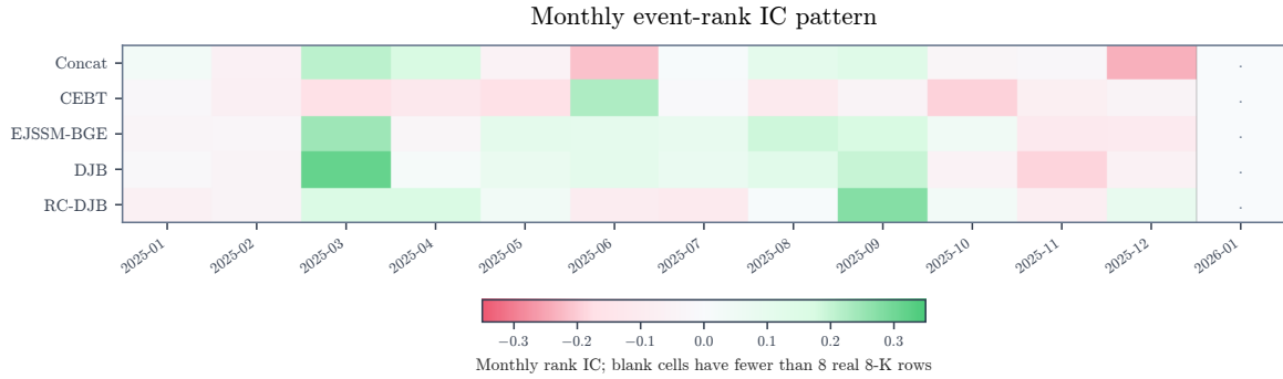
Figure A.4: Monthly event-rank IC over held-out real 8-K rows. The model-level rank result is not uniform across months, motivating ticker-clustered intervals and leave-one-ticker-out stability checks rather than a single unqualified rank statistic.
