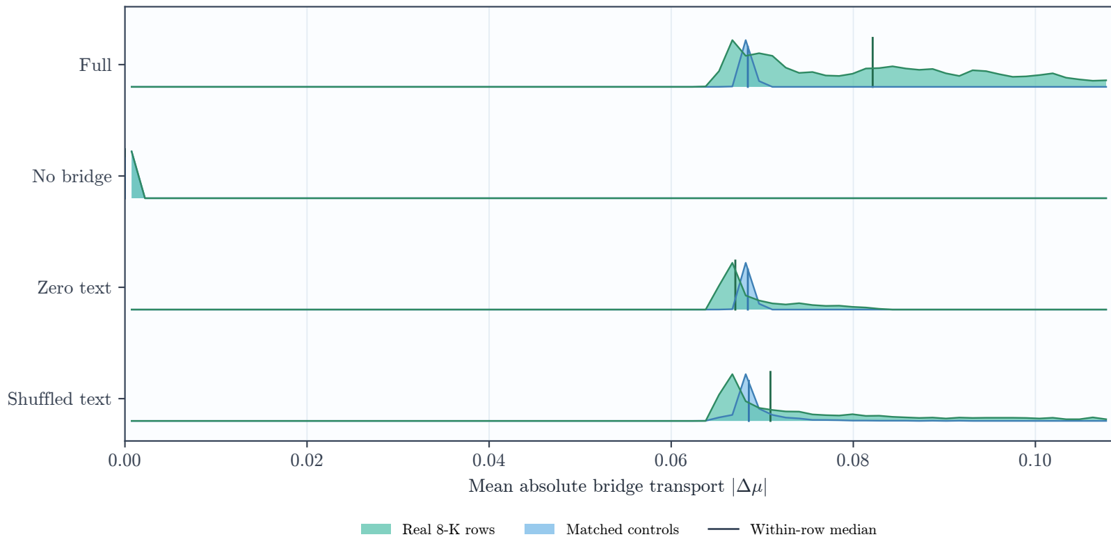
Response-transport fingerprints under interventions
