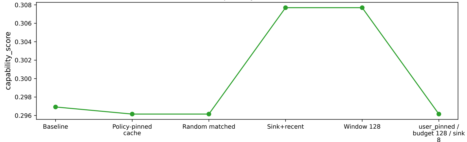
Capability Score
