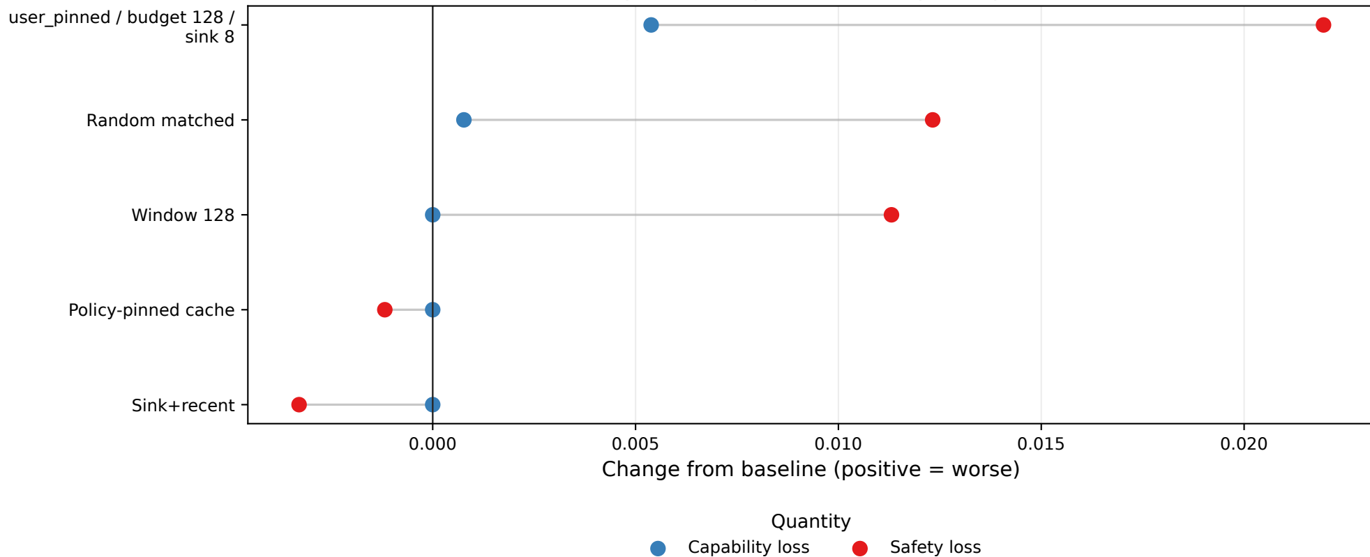
Safety loss compared with capability loss
