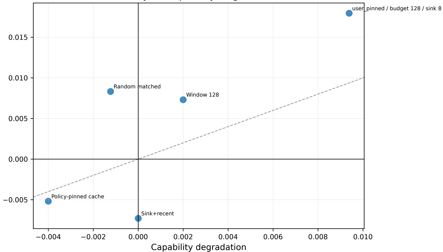
Safety vs Capability Degradation
