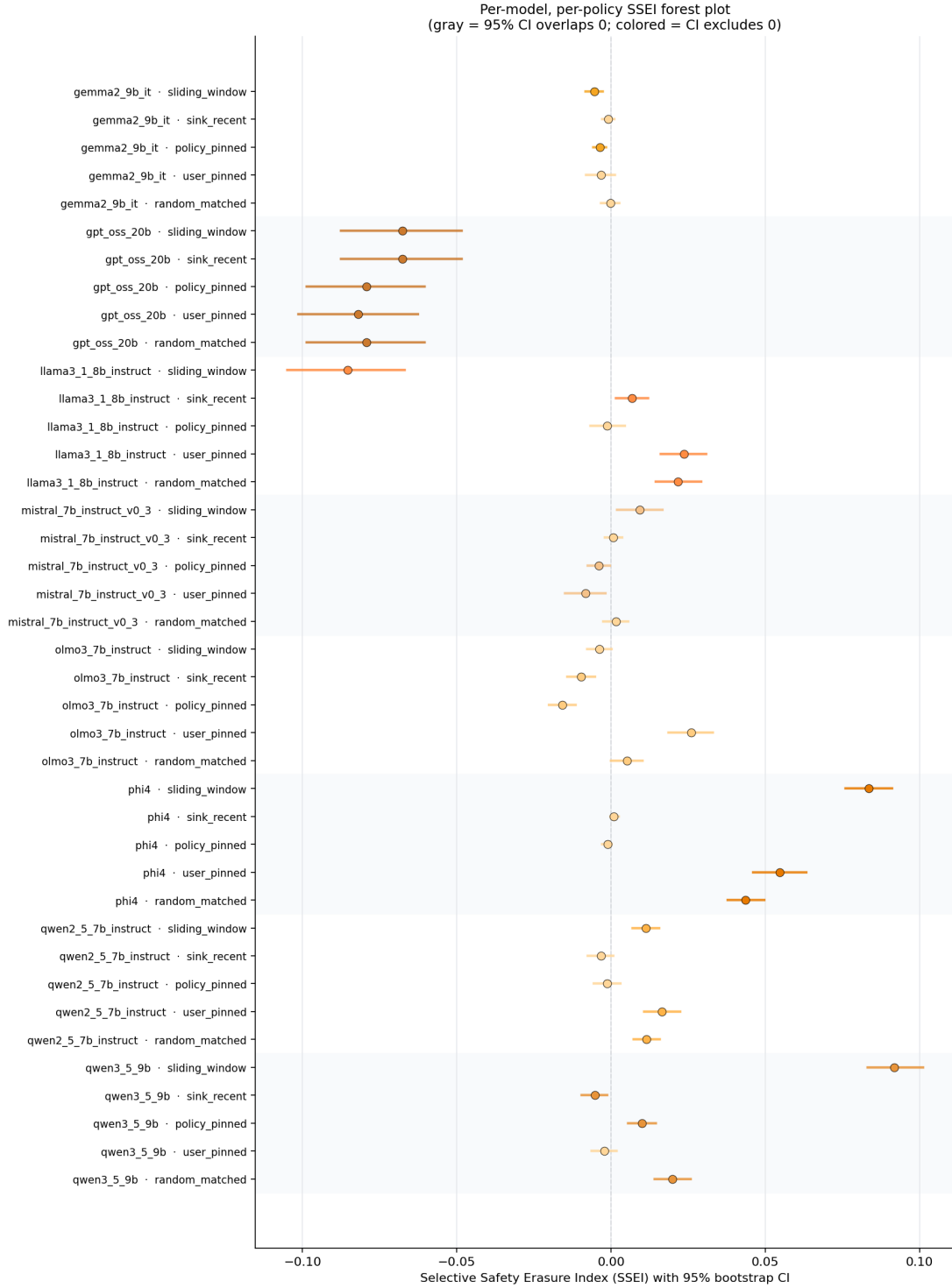
Figure 1: Selective Safety Erasure Index by model and cache policy. Each row is one (model, policy) condition; the horizontal bar is the 95% bootstrap CI and the marker is the point estimate. Light-colored rows have CIs overlapping zero; darker rows have CIs excluding zero. Four families show at least one positive condition.
