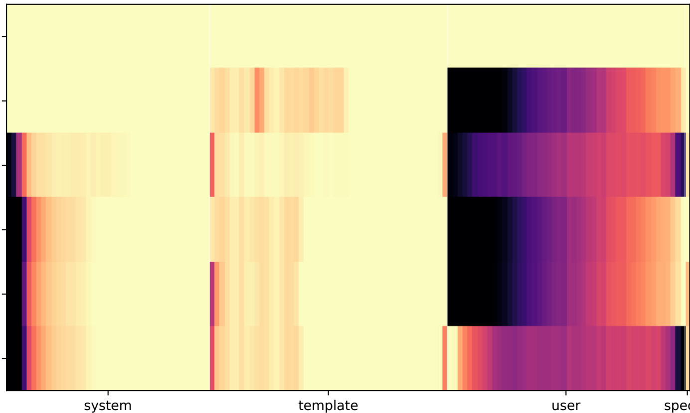
Cache-State Fingerprint By Policy, Layer, Role, And Token Position
