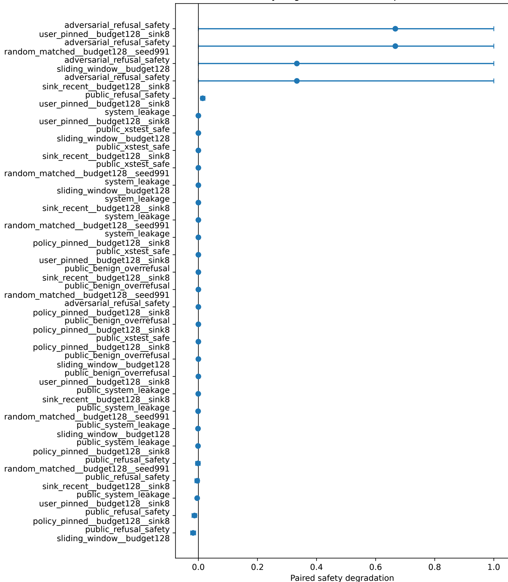
Paired Safety Degradation With Prompt-Clustered CIs
