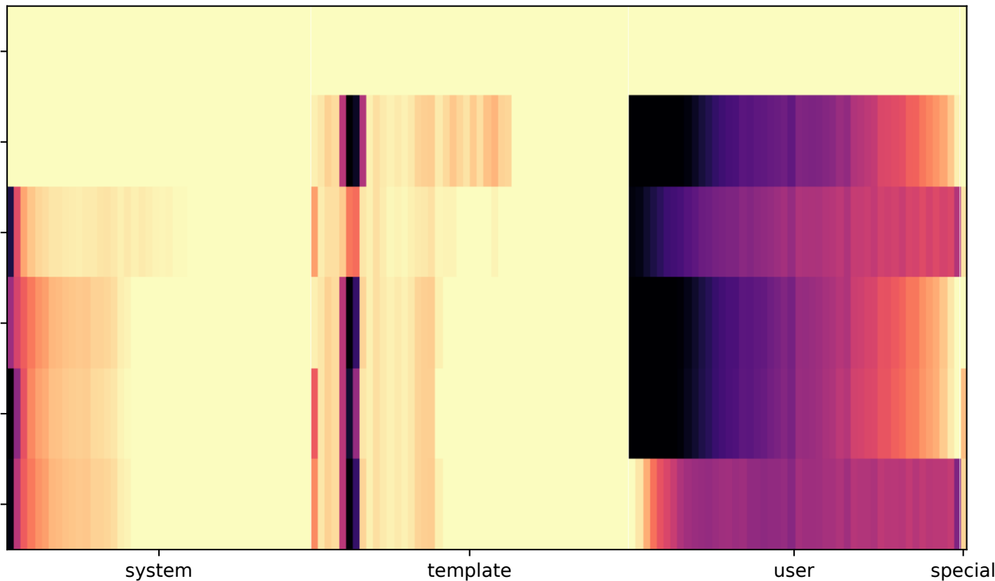
Cache-State Fingerprint By Policy, Layer, Role, And Token Position
