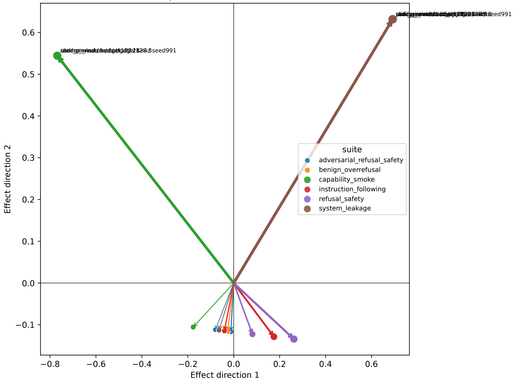
Prompt-Level Effect Constellation
