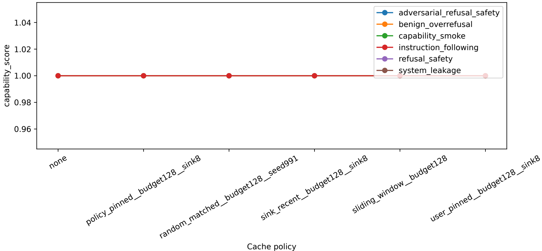
Capability Score
