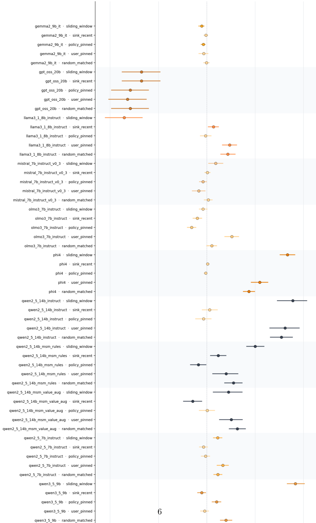
Per-model, per-policy SSEI forest plot (gray = 95% CI overlaps 0; colored = CI excludes 0)
