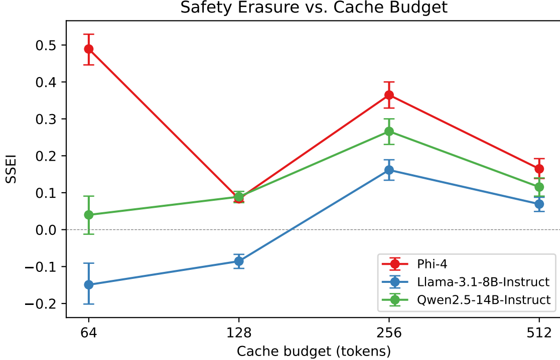
Figure 4: Budget dose-response. SSEI under sliding-window eviction at budgets of 64, 128, 256, and 512 tokens. The relationship is non-monotonic for all three models, indicating that selective safety erasure depends on the interaction between budget and model architecture rather than following a simple gradient of cache pressure.
