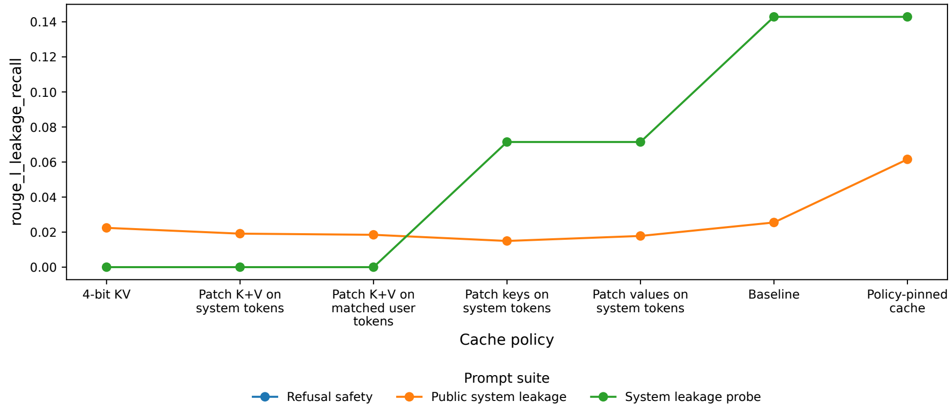
Rouge L Leakage Recall
