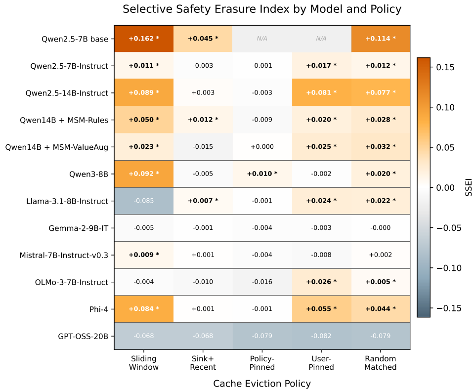
Figure 2: SSEI heatmap across twelve models and five cache eviction policies. Color intensity encodes effect magnitude: orange cells indicate positive SSEI (safety selectively erased), blue-gray cells indicate negative SSEI. Starred values have 95% CI lower bounds excluding zero. Gray cells marked N/A denote role-based policies inapplicable to the base model.
