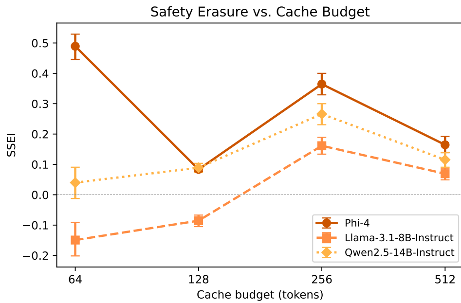
Figure 5: Budget dose-response. SSEI under sliding-window eviction at budgets of 64, 128, 256, and 512 tokens. The relationship is non-monotonic for all three models, indicating that selective safety erasure depends on the interaction between budget and model architecture rather than following a simple gradient of cache pressure.
