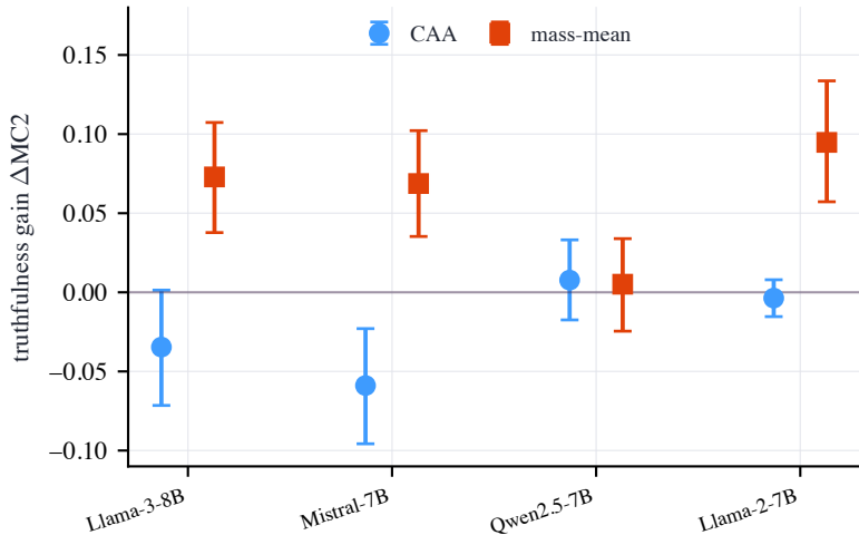
(a) Steering effect across models
