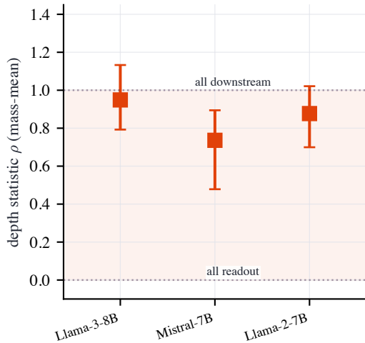
(b) Depth where effect is real
