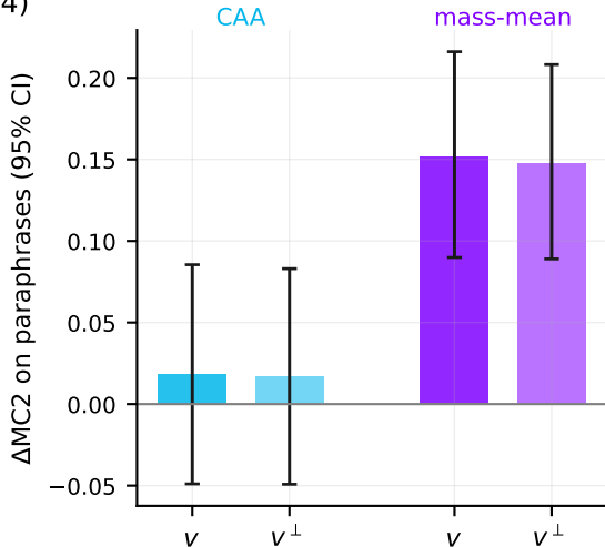
out-of-distribution (paraphrases)
