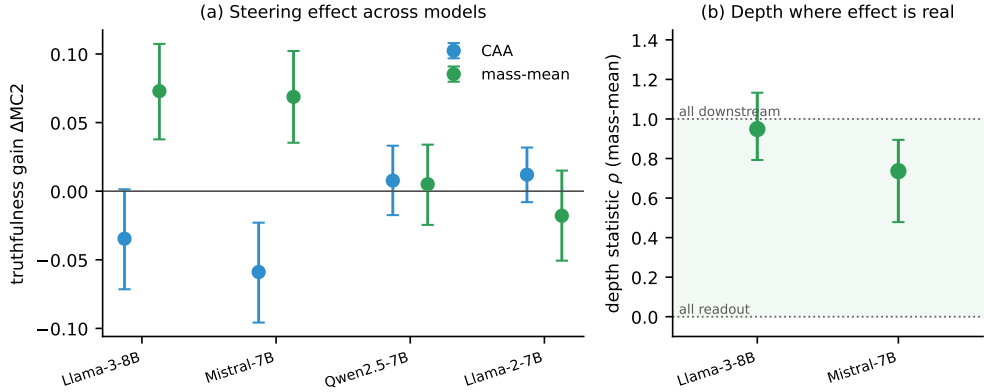
Figure 7: (a) The steering effect itself, \Delta\text{MC2} on held-out TruthfulQA, for both families across all four models (95% intervals). CAA (blue) never improves truthfulness: it is significantly negative on Mistral and indistinguishable from zero elsewhere. The mass-mean effect (green) is significantly positive on Llama-3 and Mistral but absent on Qwen and Llama-2. (b) The depth statistic \rho for the mass-mean construction, shown only for the two models where the effect is a significant truthfulness gain. On both, \rho sits in the upper, predominantly-downstream band rather than near the \rho \approx 0 that pure vocabulary suppression predicts. The other cases are omitted from (b) because \rho decomposes a gain, and there is none to decompose: CAA produces no gain on any model, and the mass-mean effect is absent on Qwen and Llama-2.
