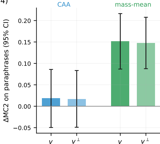
out-of-distribution (paraphrases)
