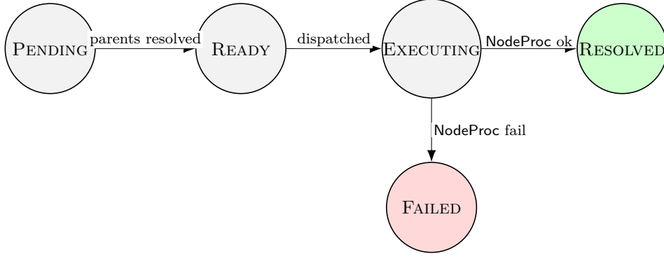
Figure 1: The node-state machine. \text{PENDING} \rightarrow \text{READY} is gated by a hard predicate on parent state; \text{READY} \rightarrow \text{EXECUTING} by dispatch; \text{EXECUTING} \rightarrow \text{RESOLVED} or \text{EXECUTING} \rightarrow \text{FAILED} by the outcome of the node-processor call.
