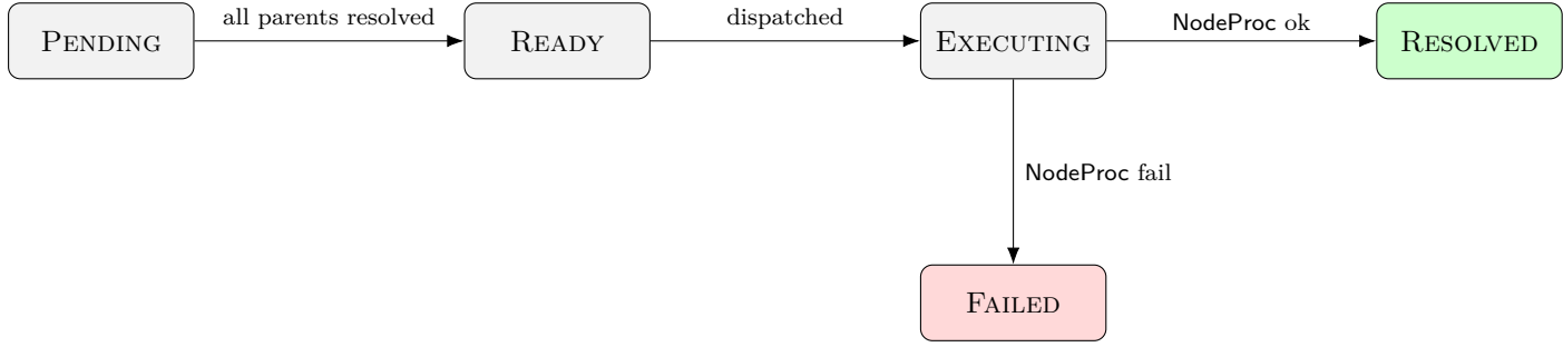
Figure 1: The node-state machine. \text{PENDING} \rightarrow \text{READY} is gated by a hard predicate on parent state; \text{READY} \rightarrow \text{EXECUTING} by dispatch; \text{EXECUTING} \rightarrow \text{RESOLVED} or \text{EXECUTING} \rightarrow \text{FAILED} by the outcome of the node-processor call.
