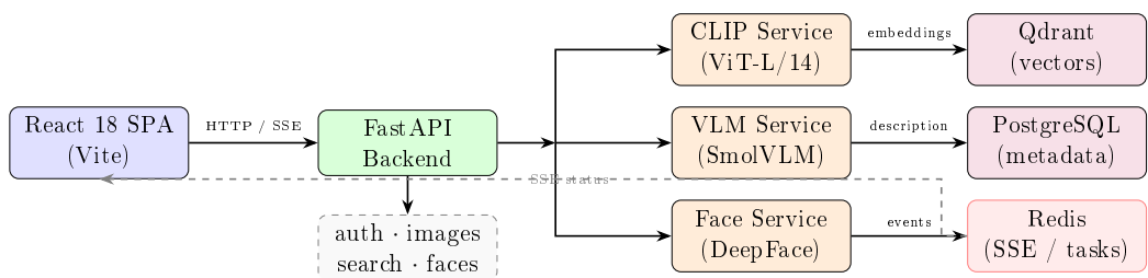
Figure 1: High-level system architecture of the AI-Powered Media Search system
