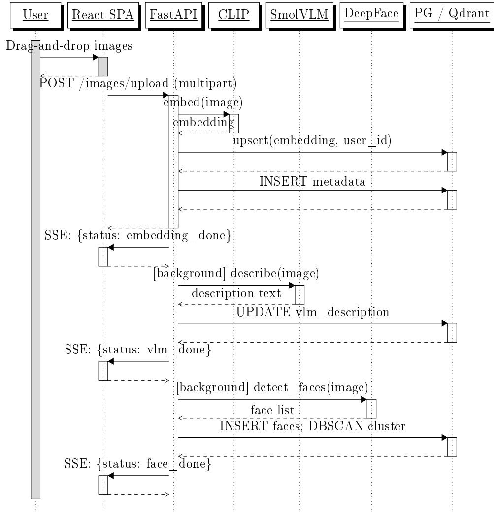
Figure 7: Sequence diagram for the image upload and background processing flow
