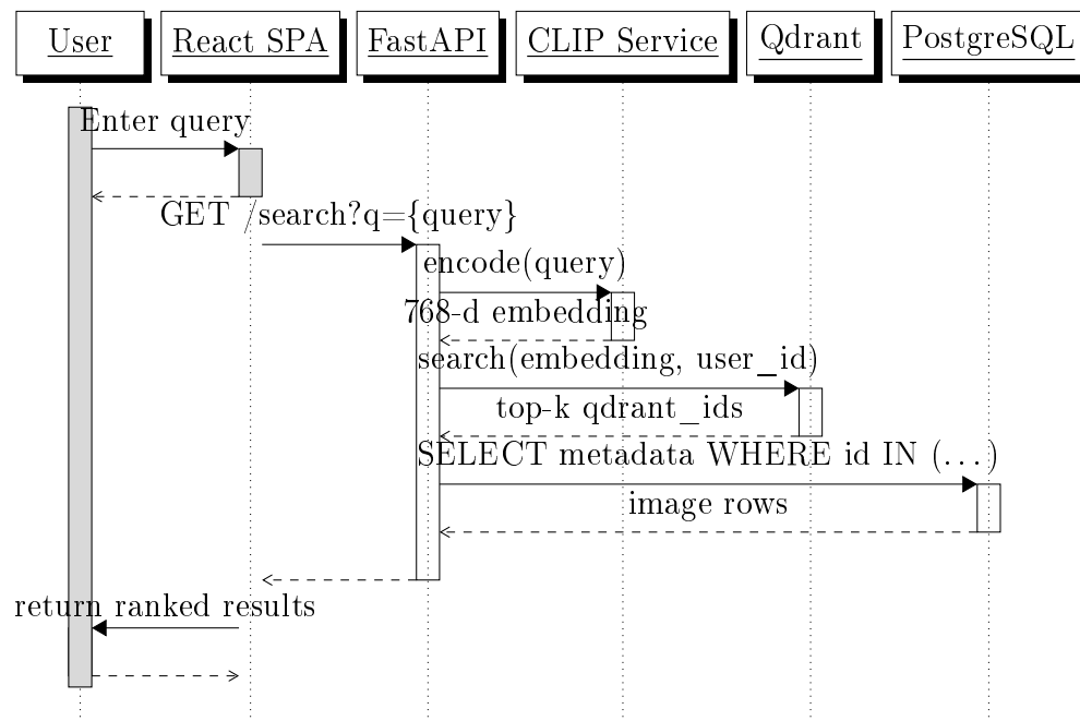
Figure 6: Sequence diagram for the semantic search flow
