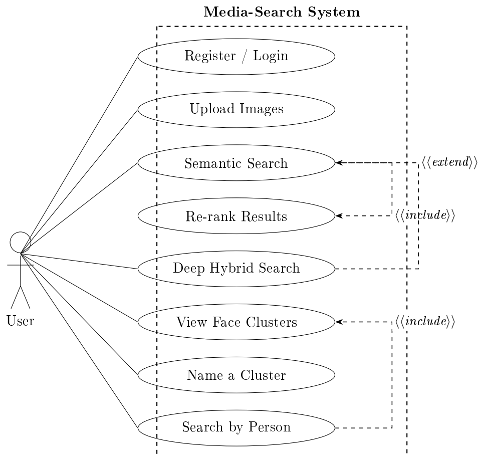
Figure 5: Use Case Diagram for the Media-Search system
