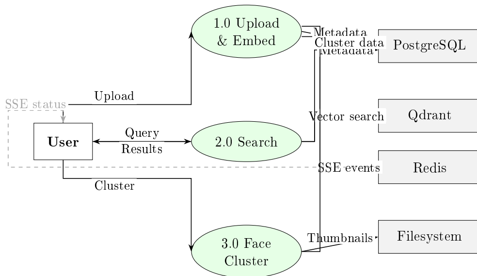
Figure 4: Level-1 DFD of the Media-Search system
