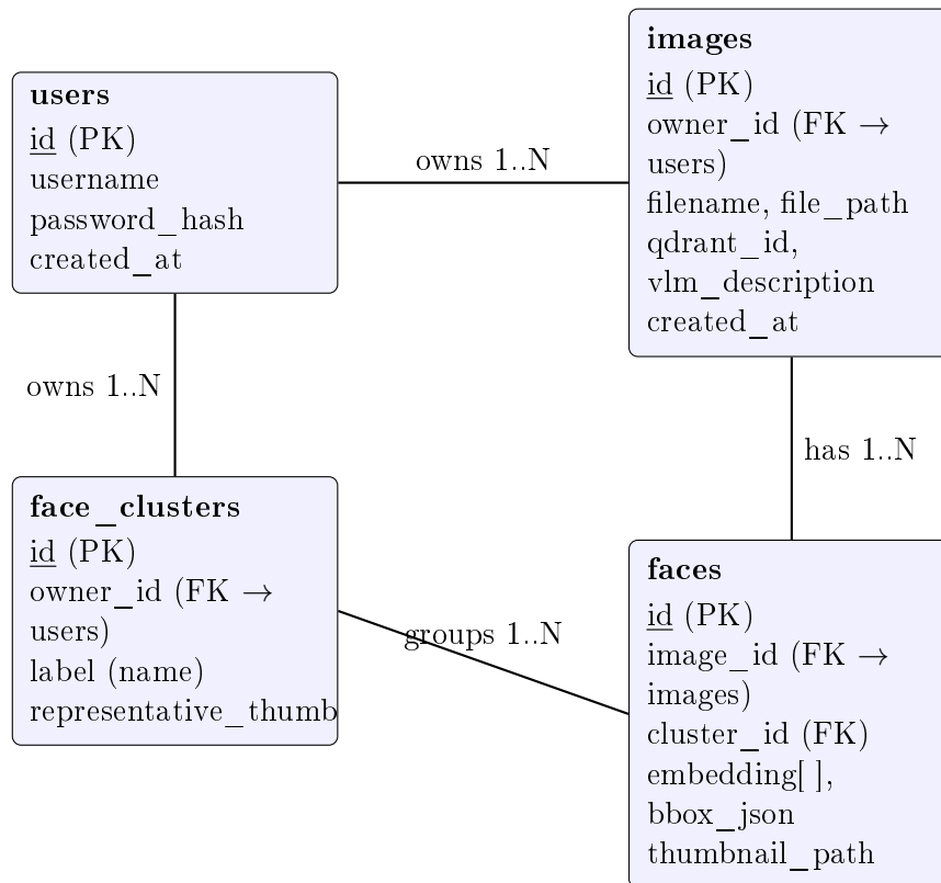
Figure 2: Entity-Relationship Diagram of the Media-Search database schema
