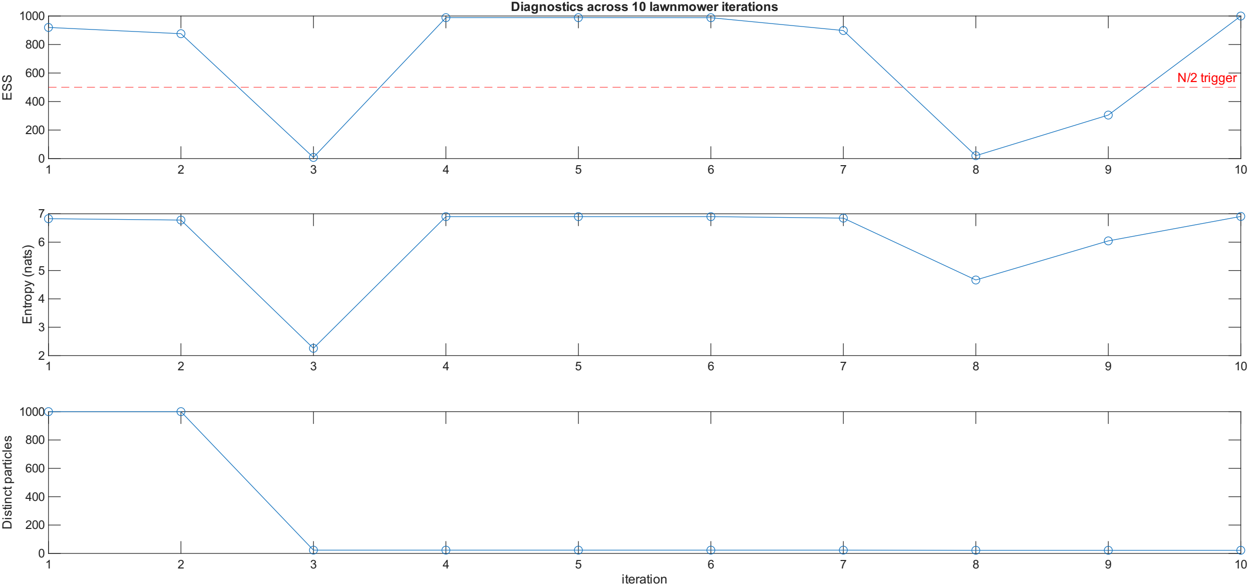
Diagnostics across 10 lawnmower iterations
