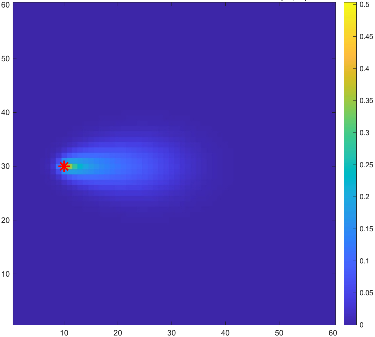
SANITY CHECK: settled field vs assumed source location (10,30)
