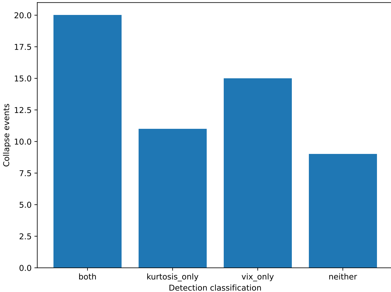
Overlap Between Kurtosis and VIX Detections
