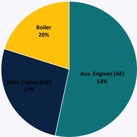
LSFO Consumption by System (46.99 MT)
