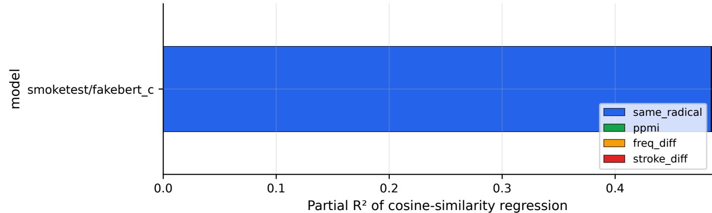
Variance decomposition of last-layer pairwise cosine
