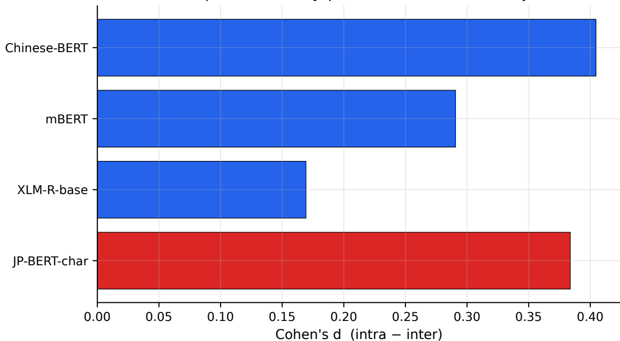
Cross-script: Chinese vs Japanese models on the kanji subset
