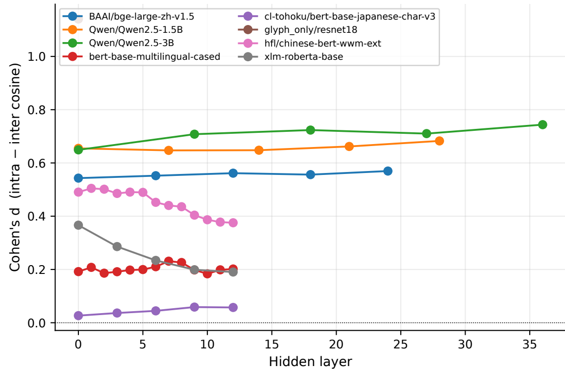
Radical-aligned cohesion across layers (char-pool, isotropy-corrected)
