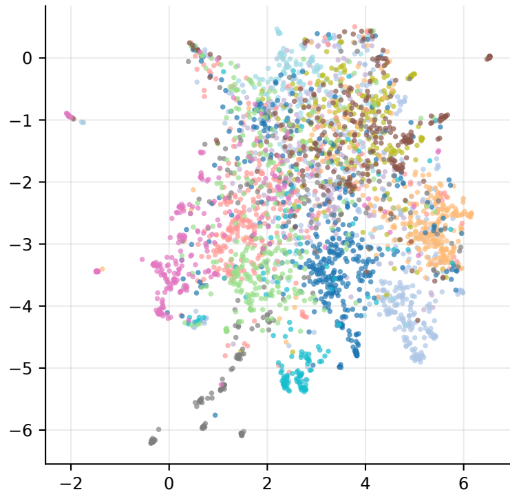
Qwen/Qwen2.5-1.5B UMAP
