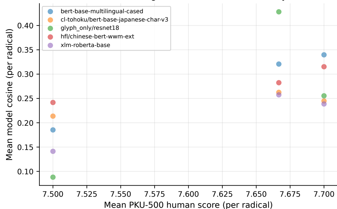
Per-radical alignment with human similarity
