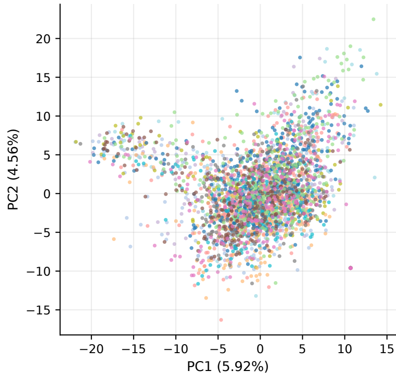
xlm-roberta-base PCA (last layer, char-pool)
