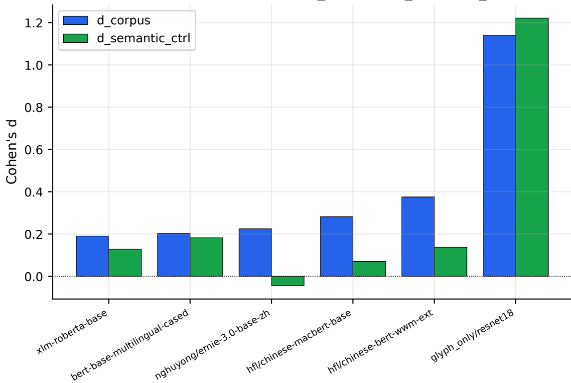
Form-specific component: d_corpus – d_semantic_ctrl
