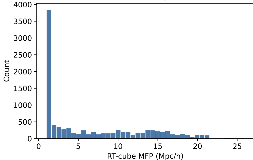
(b) RT-cube MFP distribution ( z=7.4985 ) Median=3.8 Mpc/h
