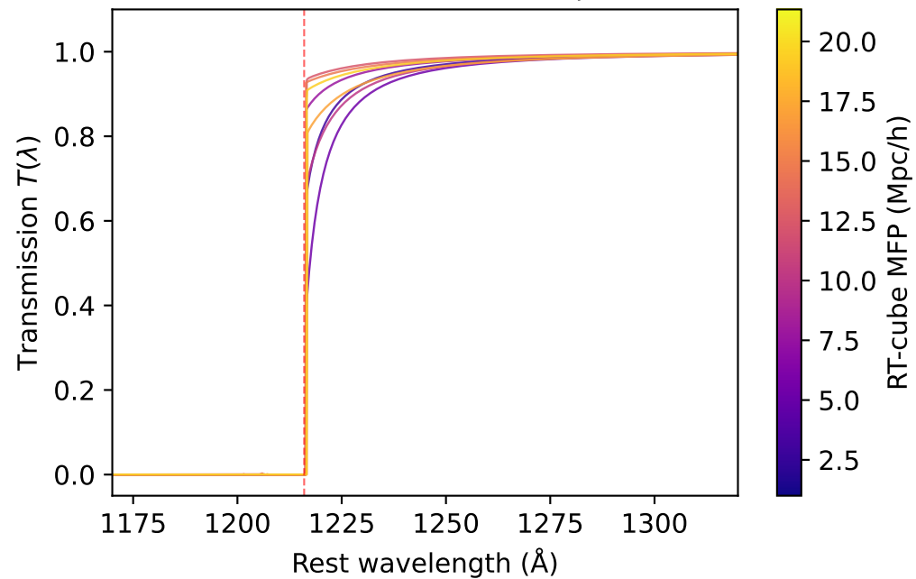
(a) Simulation transmission spectra
