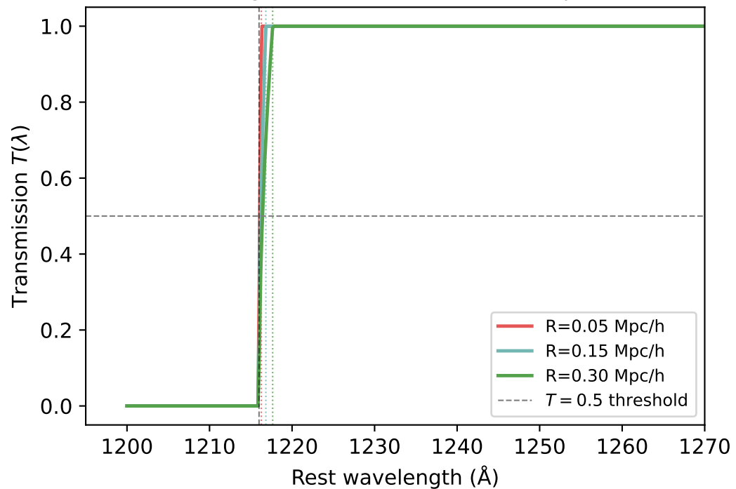
(b) How R_{\text{edge}} is read off T(\lambda) — target is a trivial feature of the input
