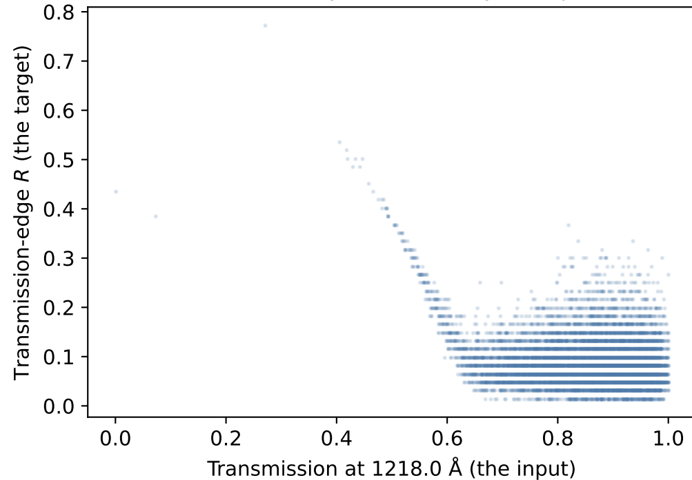
(a) Target vs input at one wavelength Pearson r = -0.217 — target is almost entirely determined by the input
