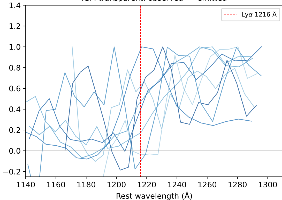
(a) Intrinsic Ly \alpha templates (JADES, z=4-5.5 ) IGM transparent: observed \approx emitted
