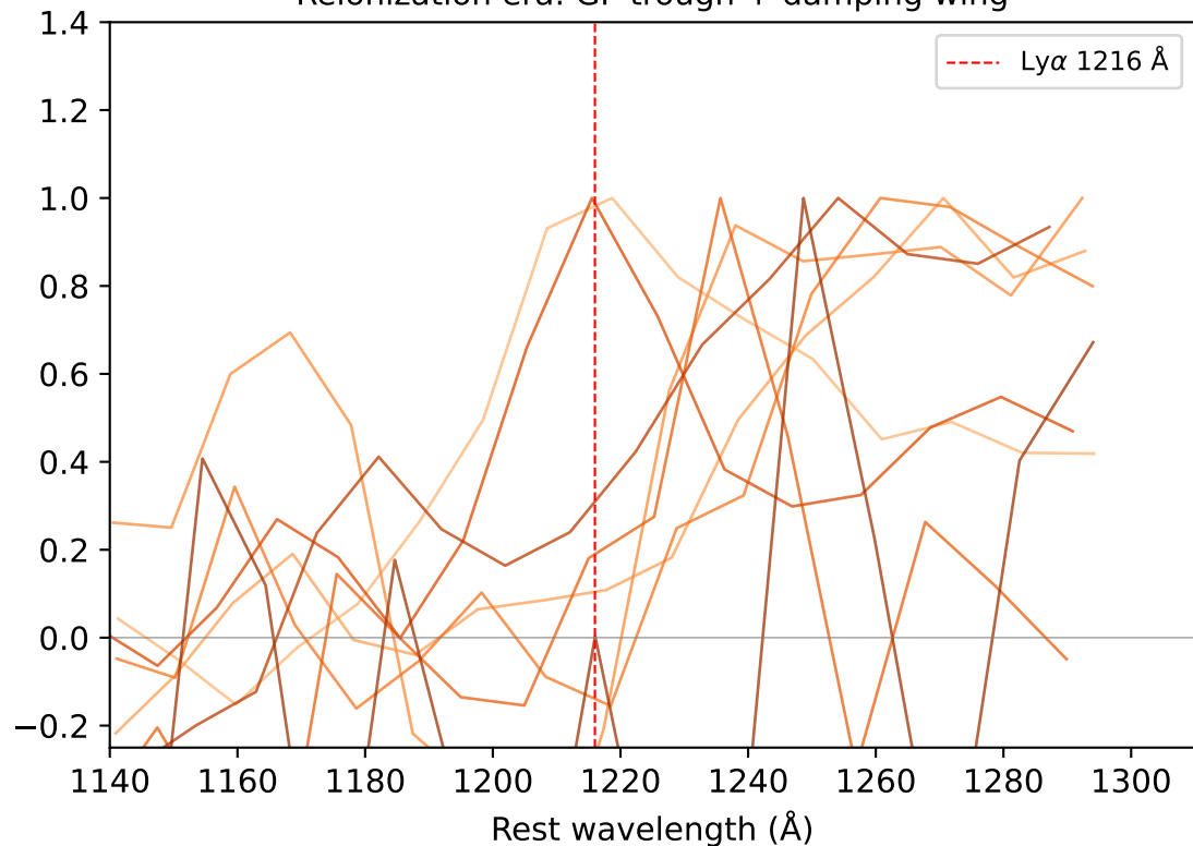
(b) Evaluation spectra (JADES, z=7-8 ) Reionization era: GP trough + damping wing
