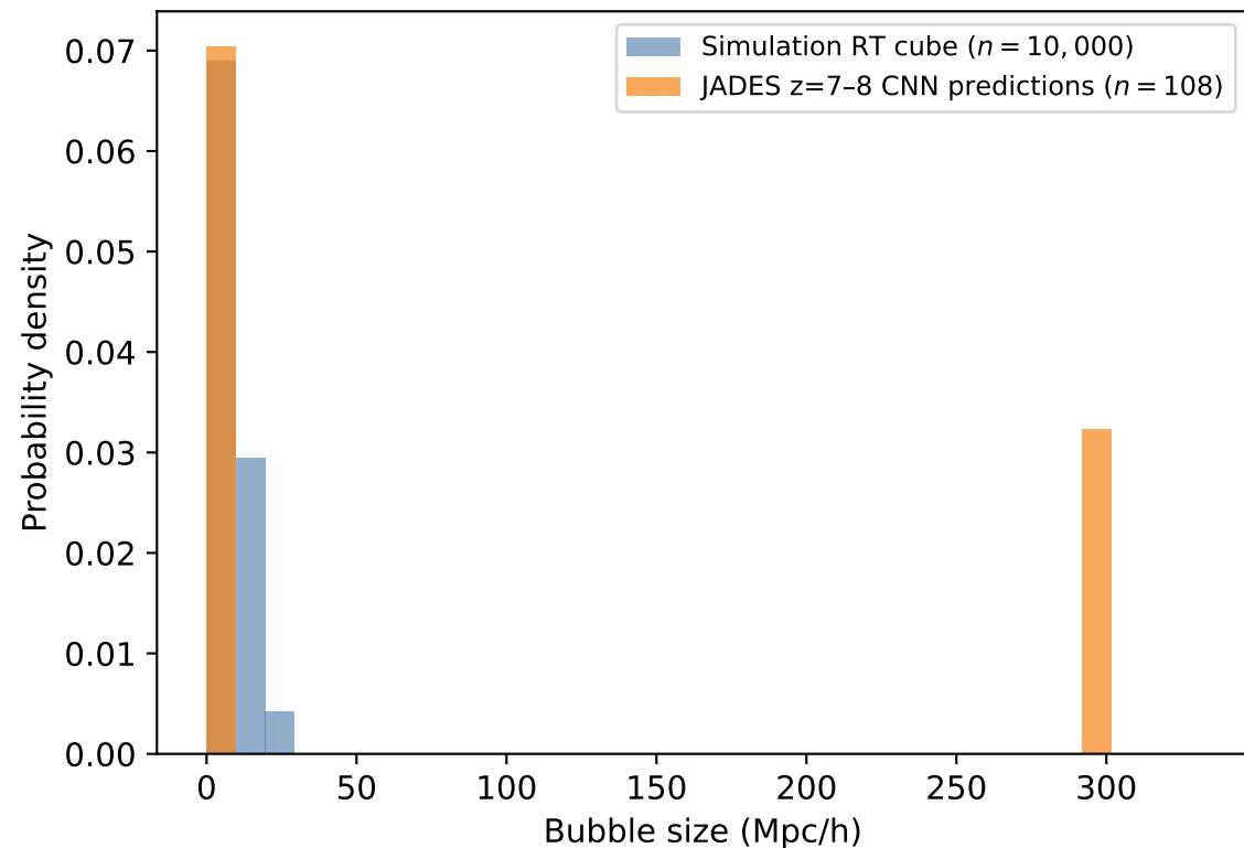
(a) Recovered bubble size distribution
