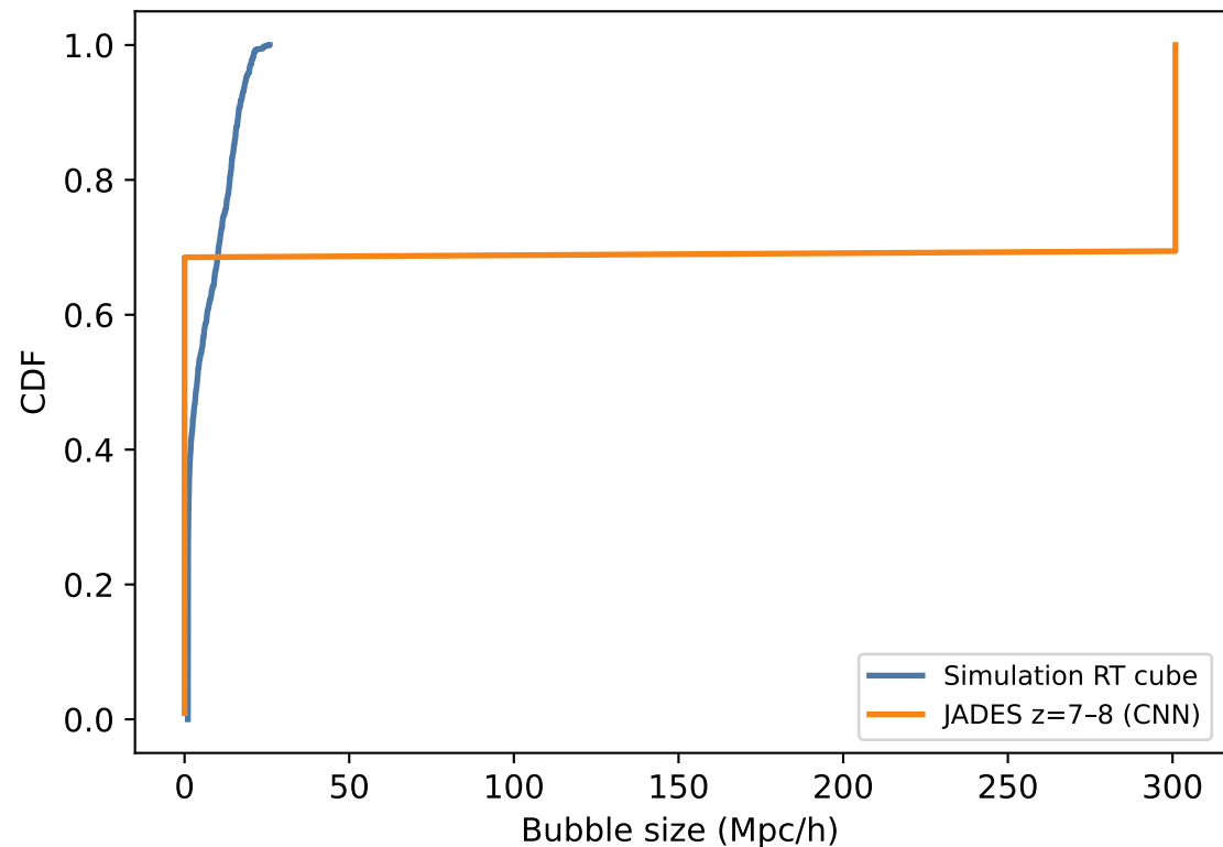
(b) Cumulative distribution KS = 0.685
