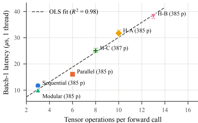
Fig. 1. Single-sample latency grows with the number of operations per call ( R^2 = 0.98 ), even though every model has about the same number of parameters.
