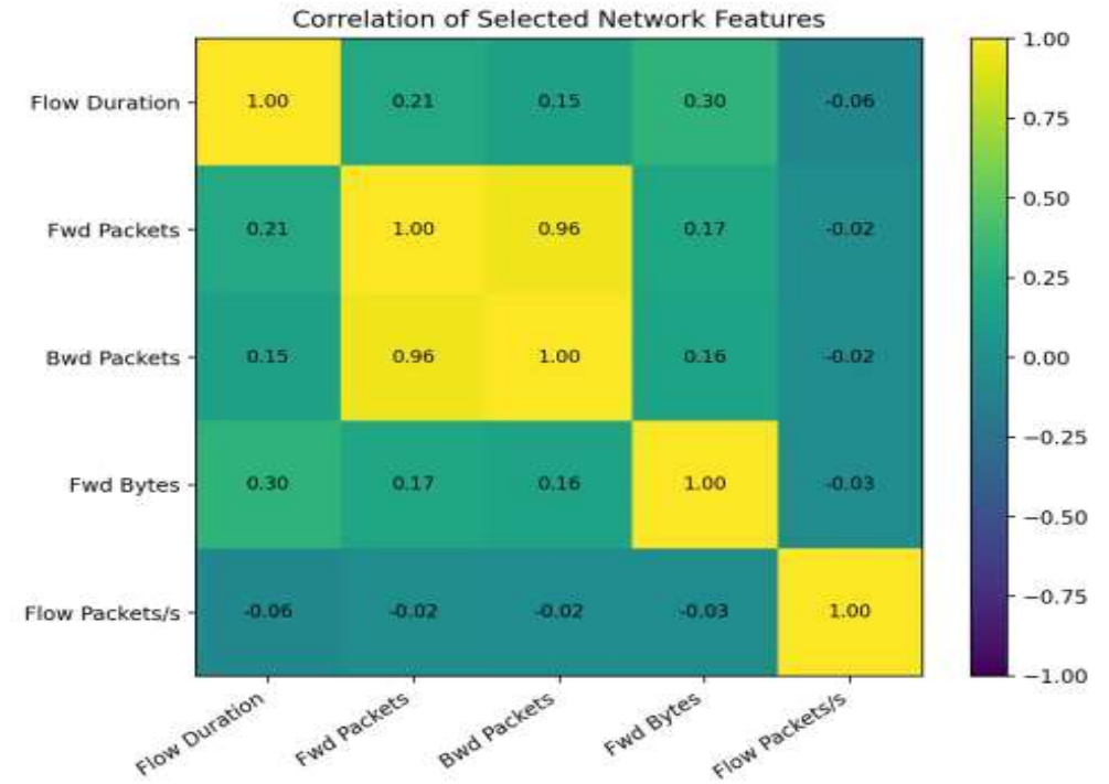
CORRELATION HEATMAP
