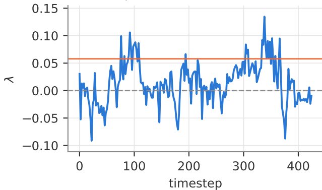
PickPlaceCounterToCab (demo 103)
