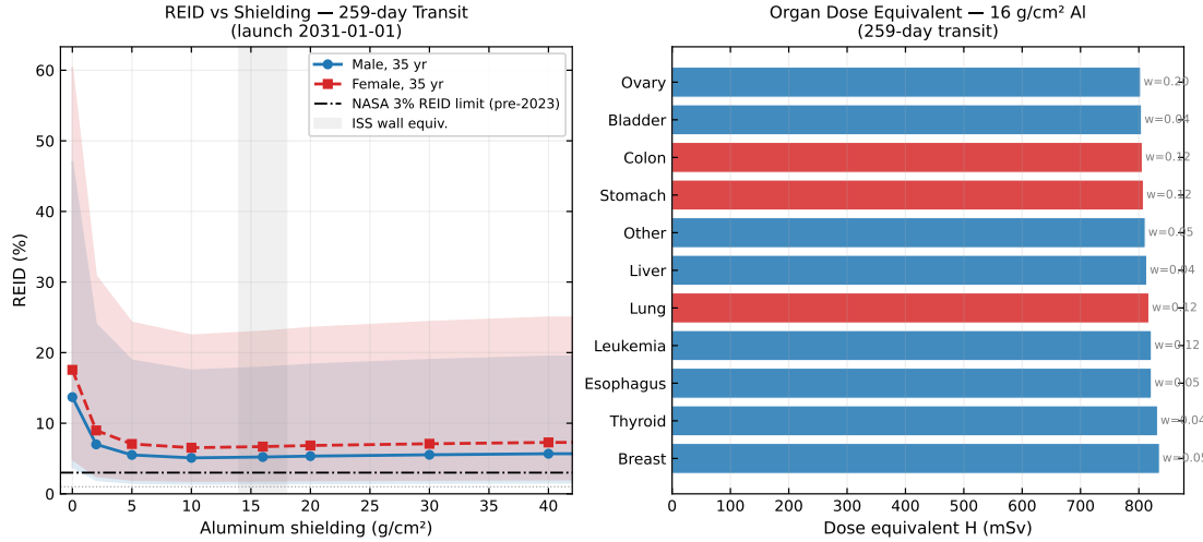
Figure 6: Left: REID (%) vs. Al shielding, male/female, p5–p95 bands; line = NASA 3% limit. Individual samples are capped at 100% (REID is a probability); the wide band below \sim 5 \text{ g cm}^{-2} reflects genuinely large compounding radiobiological uncertainty at high unshielded dose, not an artifact. Right: organ dose equivalent at 16 \text{ g cm}^{-2} Al, w_T annotated.
